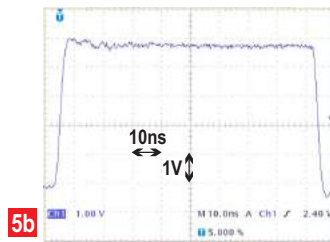
Extended pulses observed at the ID101-20 or ID101-SMF20 (5a) and ID101-50 or ID101-MMF50 or ID101-MMF100(5b) outputs at high illumination level. When an avalanche is triggered during the recharge process, the output remains high, giving an extended pulse. This effect leads to a decrease of the output count rate.
