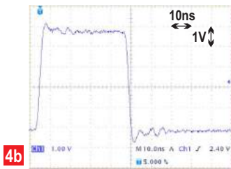
Typical pulses observed at the ID101-20 or ID101-SMF20 (4a) and ID101-50 or ID101-MMF50 or ID101-MMF100 (4b) outputs in high impedance.
