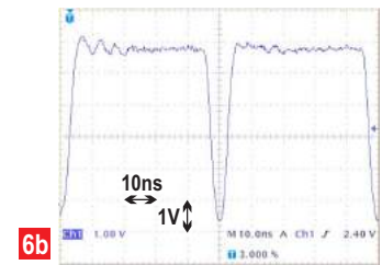
The short dead time of the ID101 allows operation at very high repetition frequencies, up to 28 MHz for the ID101-20 or ID101-SMF20 (6a) and 22 MHz for the ID101-50 or ID101-MMF50 or ID101-MMF100 (6b).
