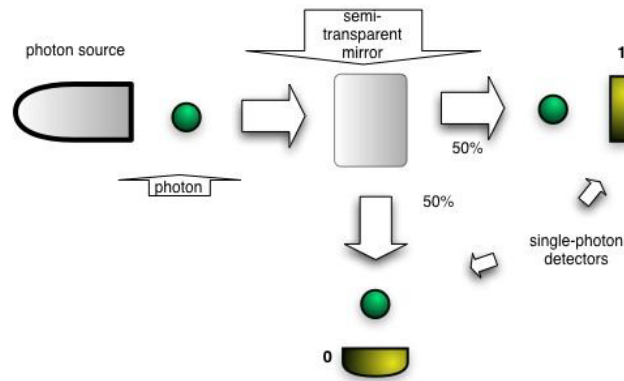
Fig. 1. Optical system for generating quantum random bits
